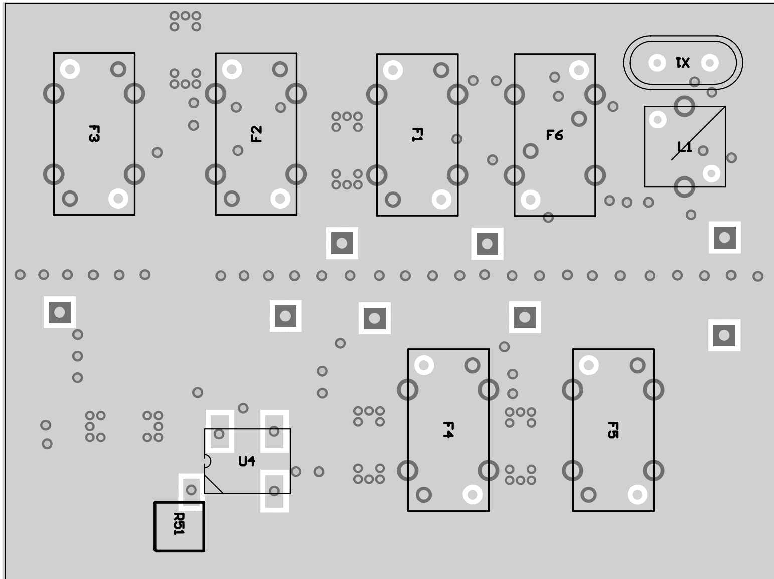
DATV – Up-Converter 70cm/13cm Version 2.0 Top Stuffing
