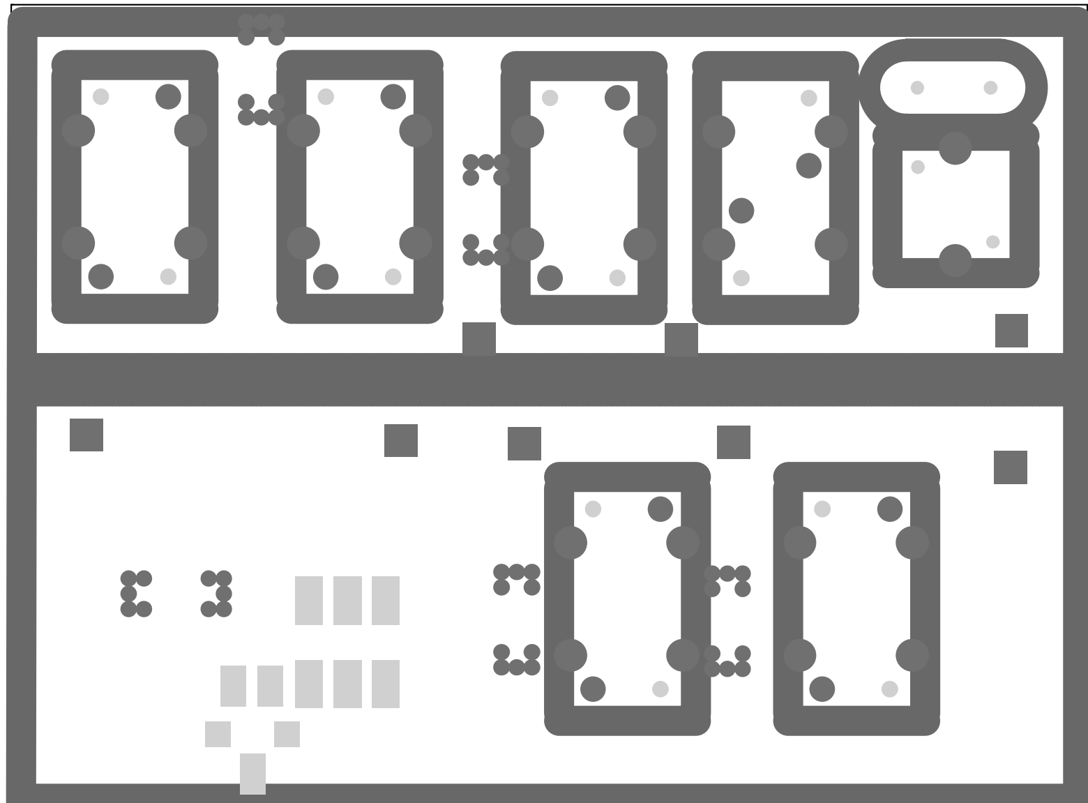
DATV – Up-Converter 70cm/13cm Version 2.0 Top Solder Mask
