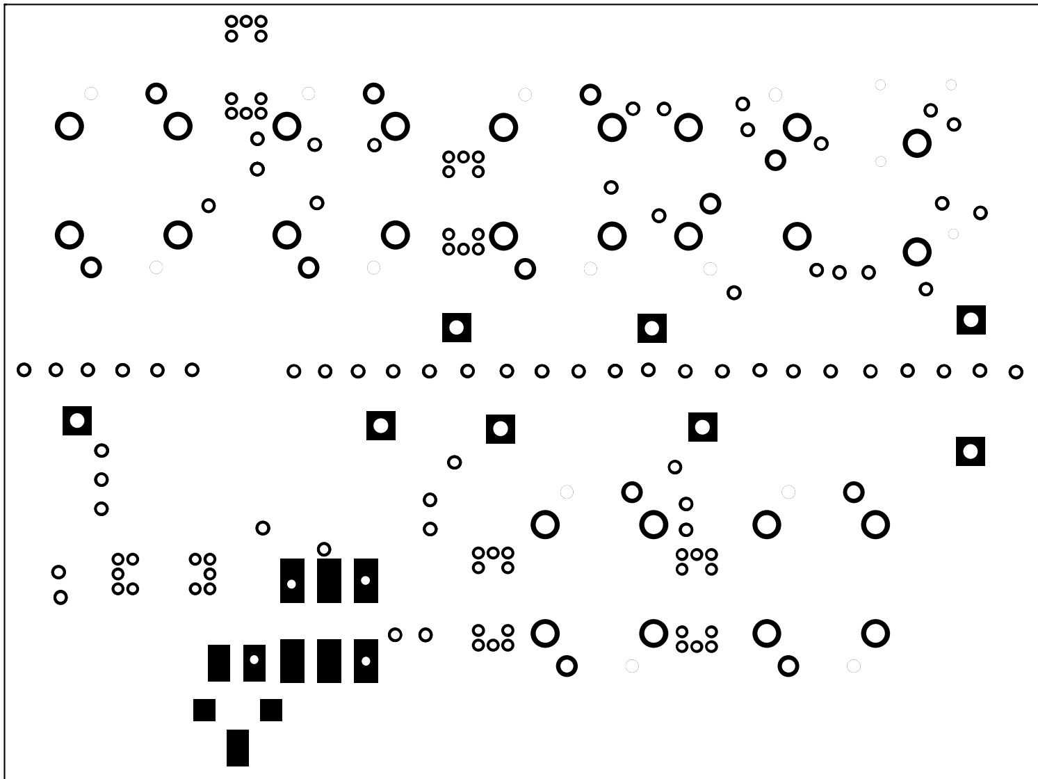
DATV – Up-Converter 70cm/13cm Version 2.0 Top Layer
