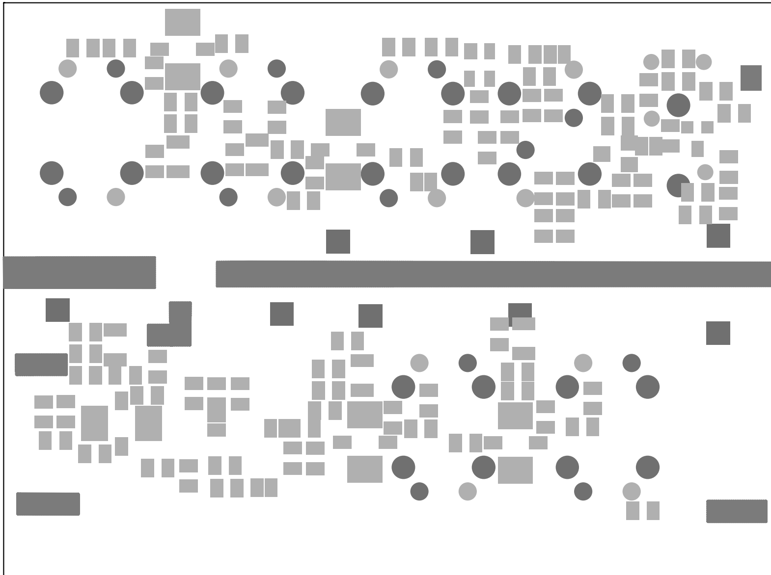
DATV – Up-Converter 70cm/13cm Version 2.0 Bottom Solder Mask
