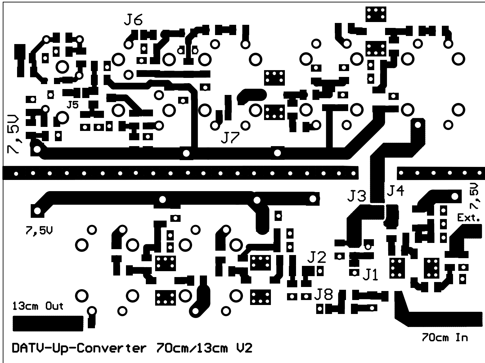
DATV – Up-Converter 70cm/13cm Version 2.0 Bottom Layer
