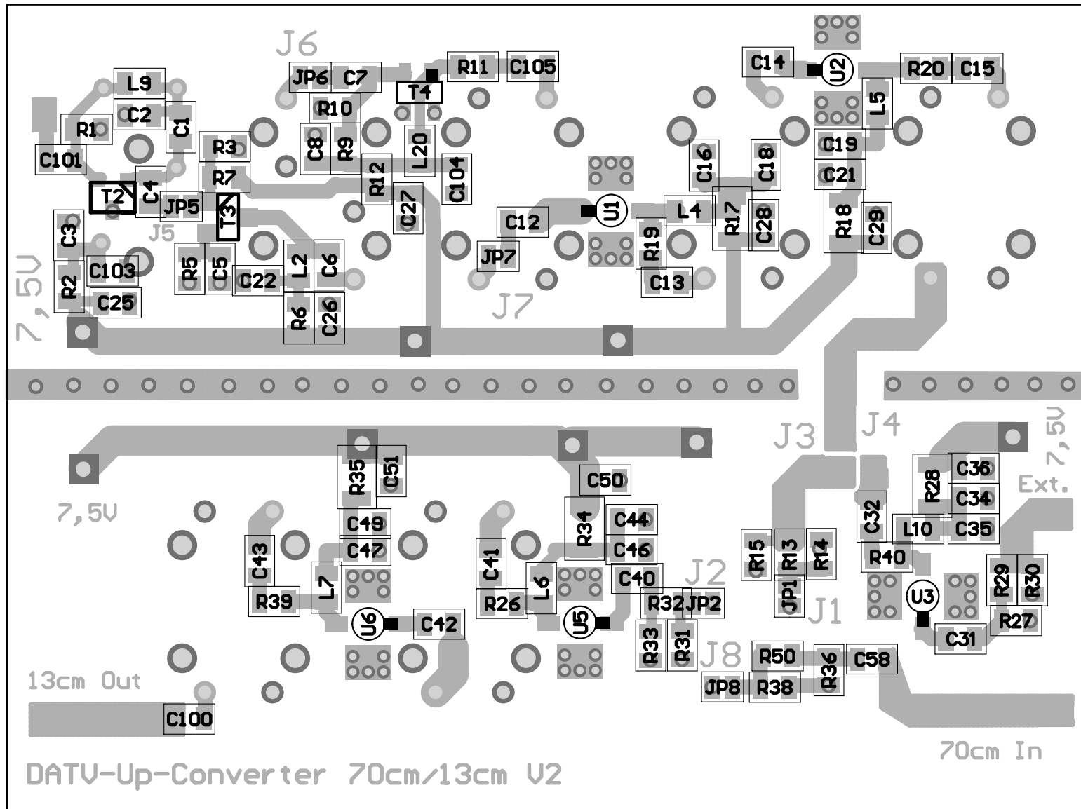
DATV – Up-Converter 70cm/13cm Version 2.0 Bottom Stuffing
