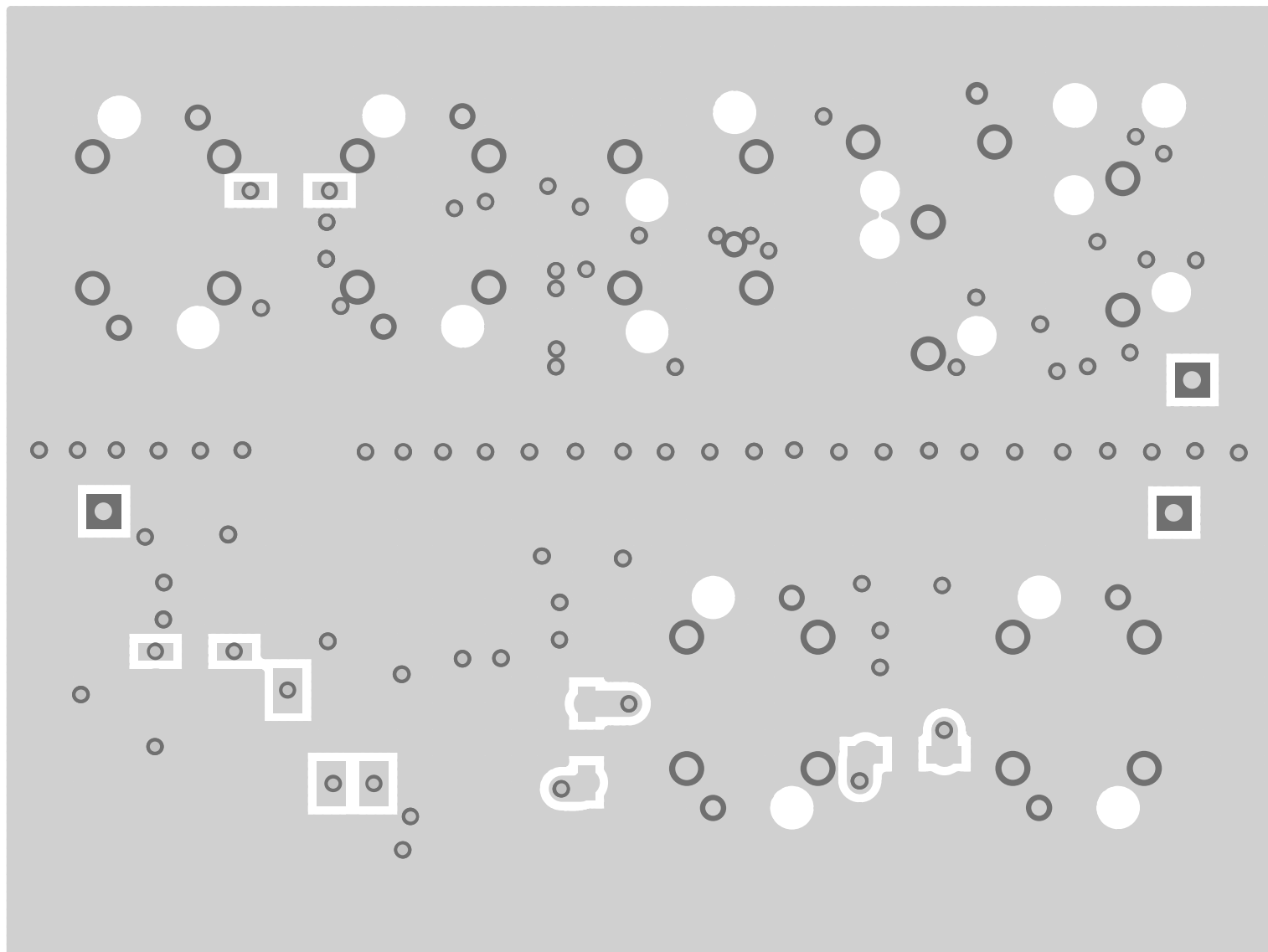
DATV – Up-Converter 70cm/23cm Version 3.4 Top Layer
