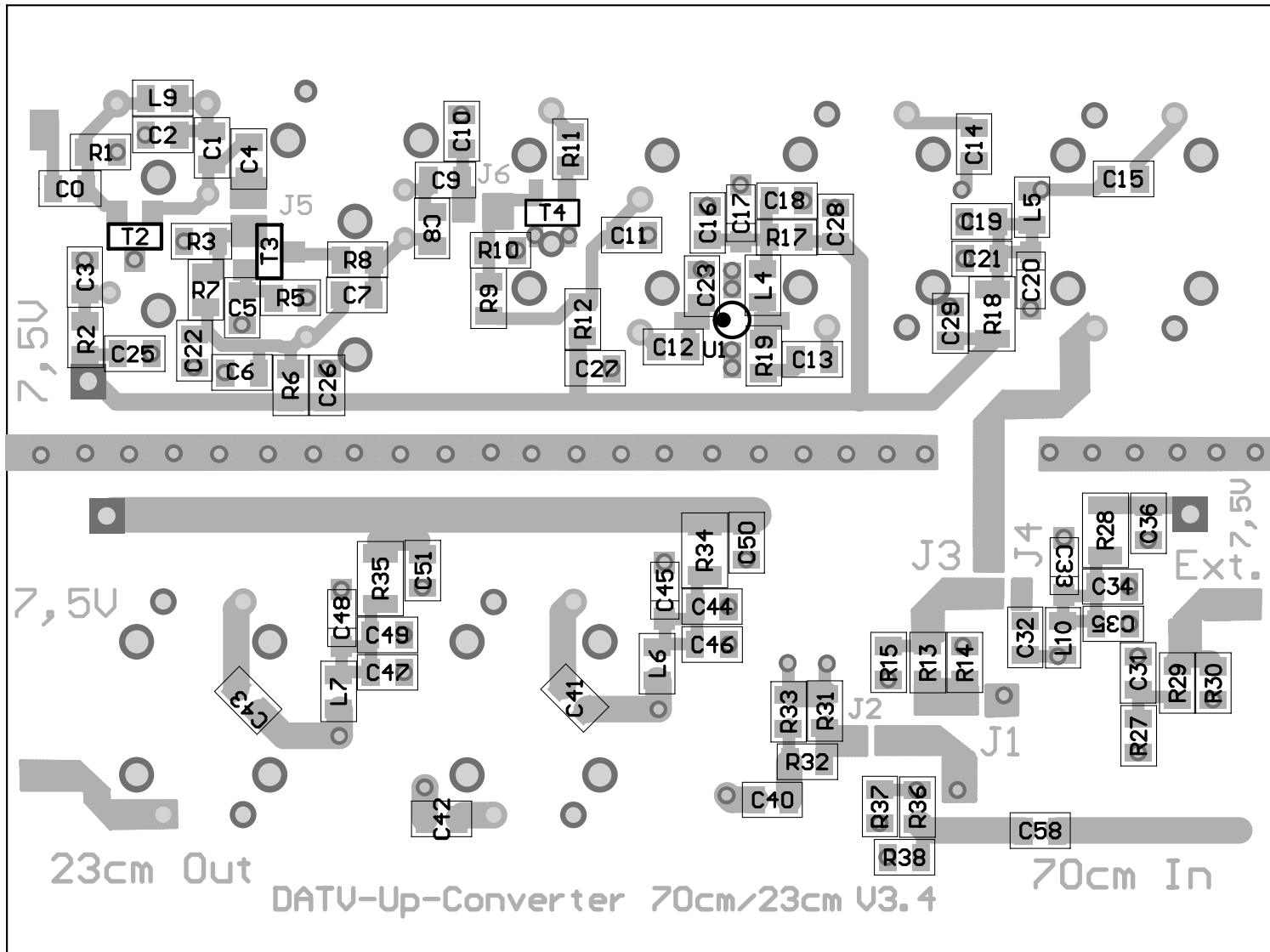
DATV – Up-Converter 70cm/23cm Version 3.4 Bottom Stuffing
