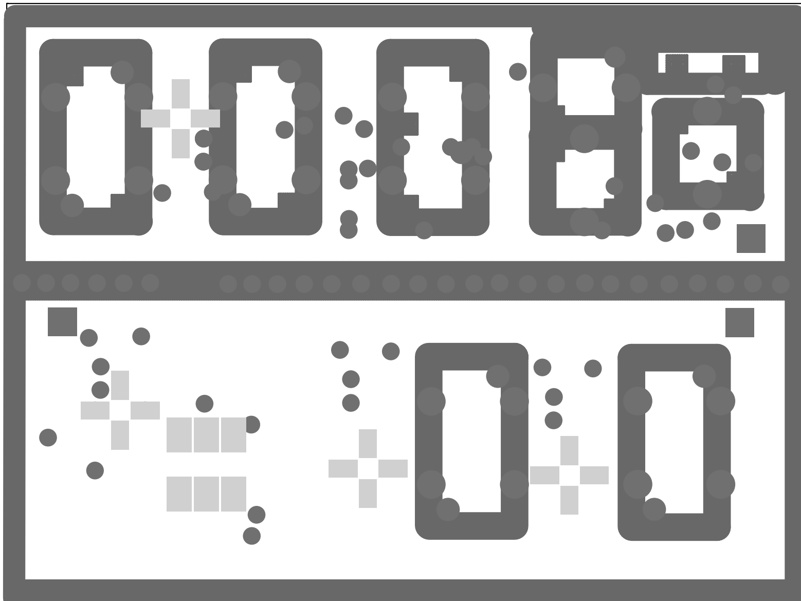
DATV – Up-Converter 70cm/23cm Version 3.4 Top Solder Mask
