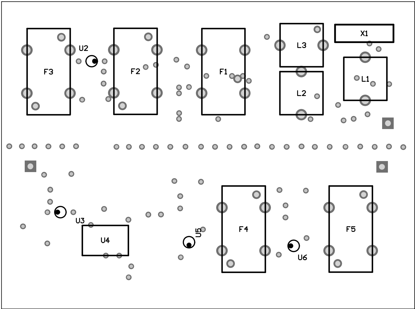
DATV – Up-Converter 70cm/23cm Version 3.4 Top Stuffing
