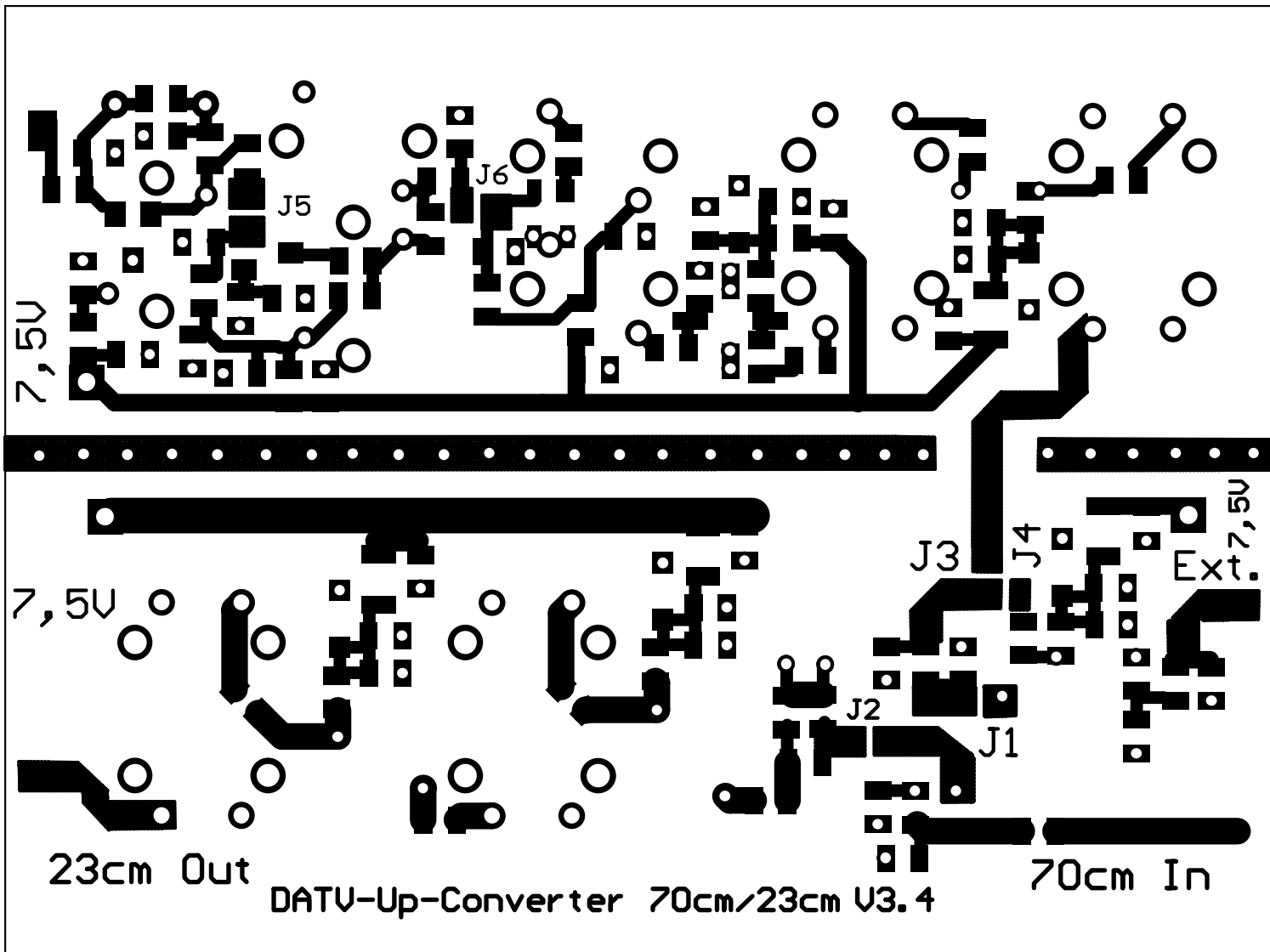
DATV – Up-Converter 70cm/23cm Version 3.4 Bottom Layer
